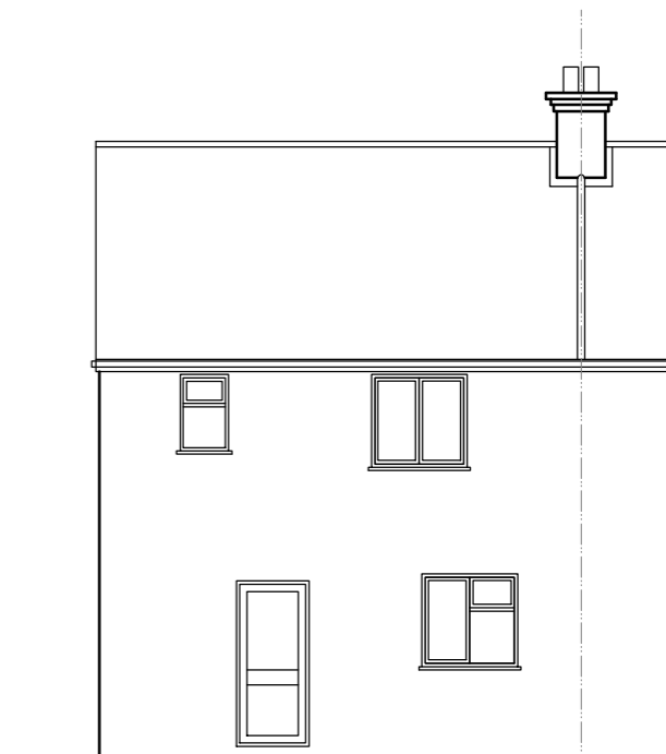
Rear Elevation
